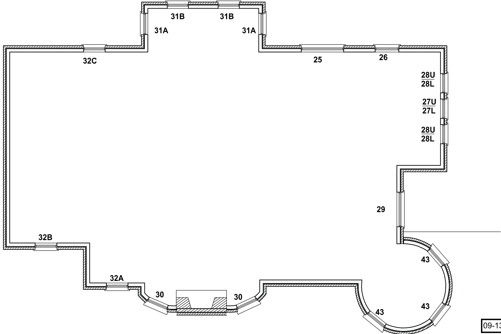
2ND FLOOR LAYOUT SCALE: 1/4" = 1'-0"
