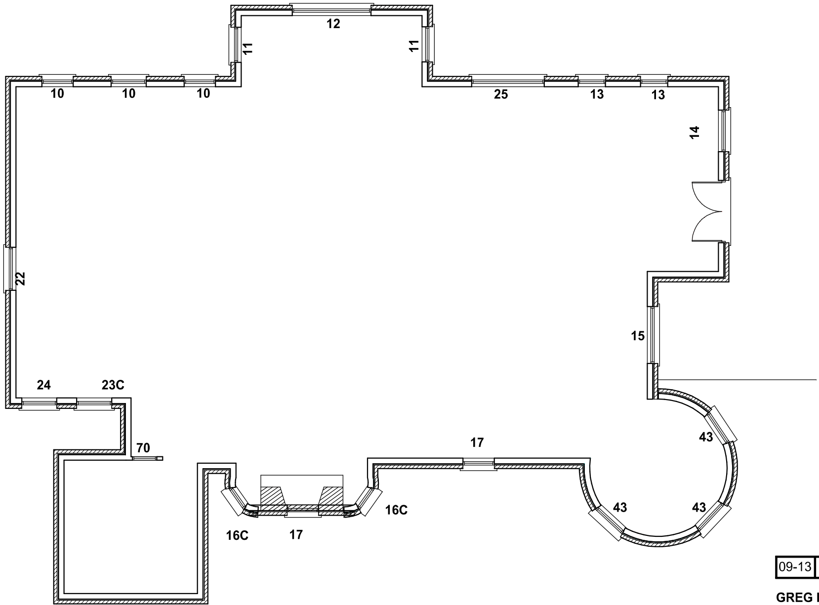
1ST FLOOR LAYOUT SCALE: 1/4" = 1'-0"
